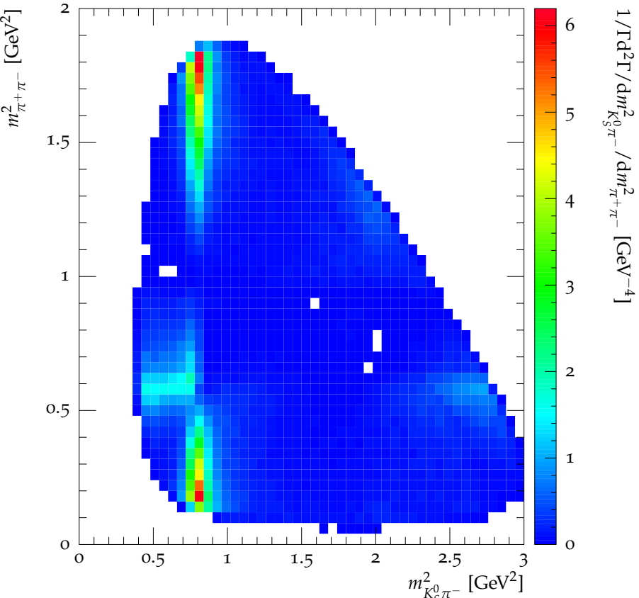
Dalitz plot for D^0 \rightarrow K_S^0 \pi^+ \pi^-
