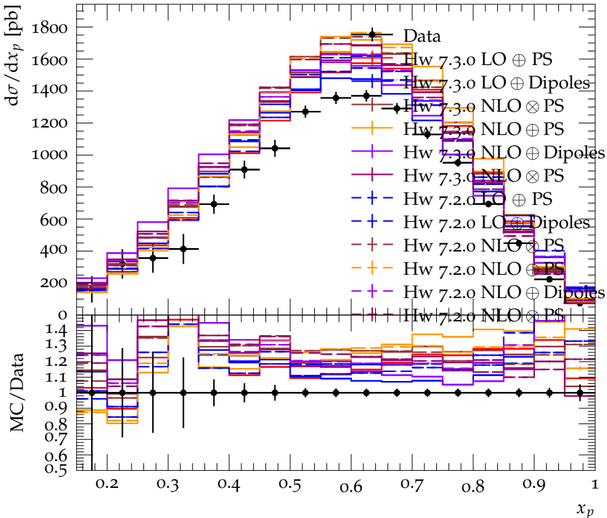
Average D meson scaled momentum distribution
