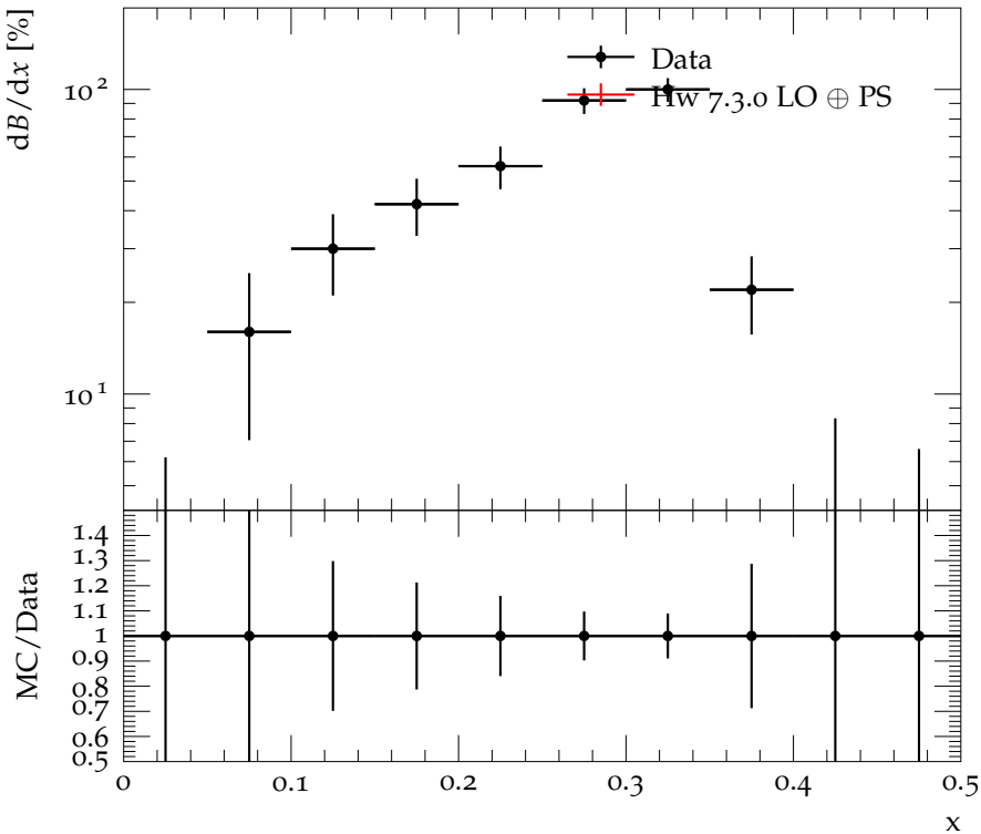
Scaled momentum spectrum of D_s^\pm mesons in Y(4S) decays
