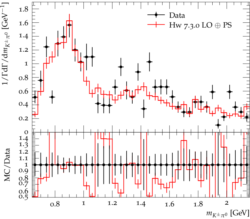
K^\pm \pi^0 mass distribution in \chi_{c0} \rightarrow K^\pm \pi^\mp K_S^0 \pi^0
