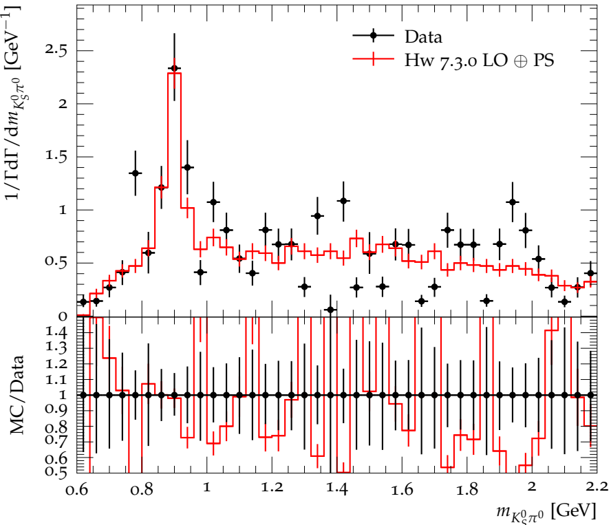
K_S^0\pi^0 mass distribution in \chi_{c2} \rightarrow K^\pm\pi^\mp K_S^0\pi^0
