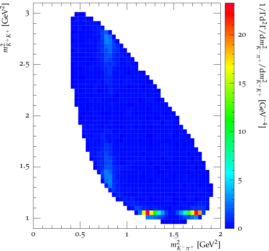
Dalitz plot for D^+ \rightarrow K^+ K^- \pi^+
