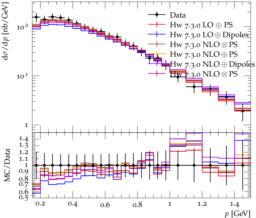
\pi^\pm momentum spectrum for E_{\text{CMS}} = 3.98 \rightarrow 4.10 GeV
