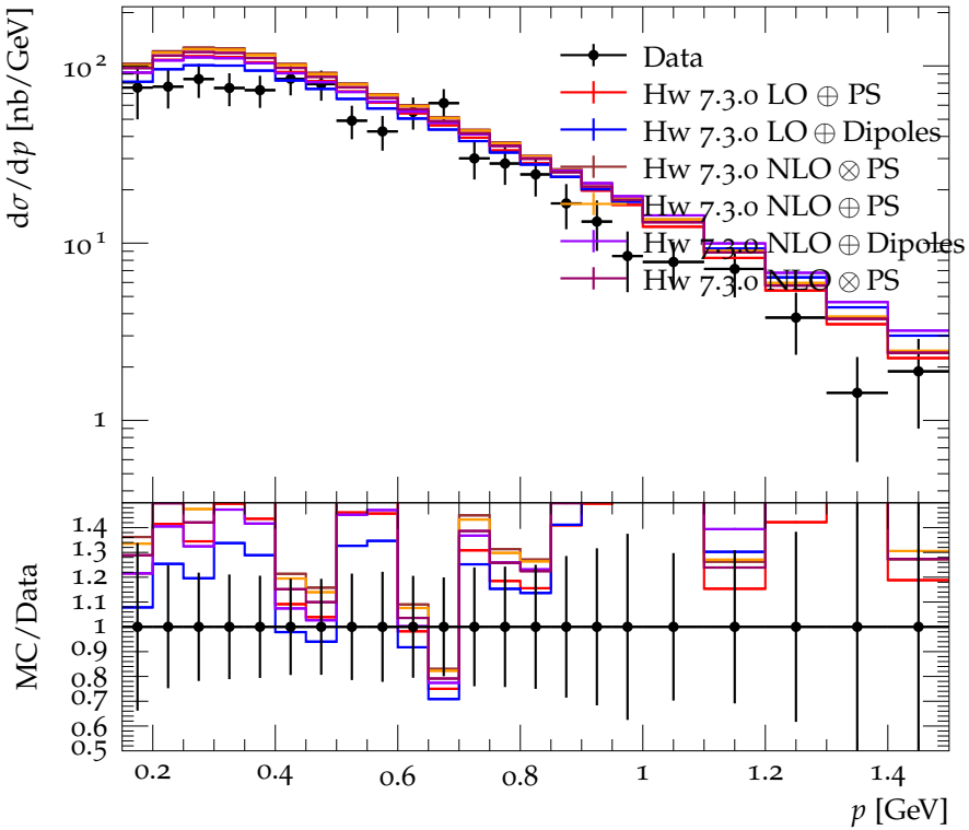
\pi^\pm momentum spectrum for E_{\text{CMS}} = 4.24 \rightarrow 4.36 GeV
