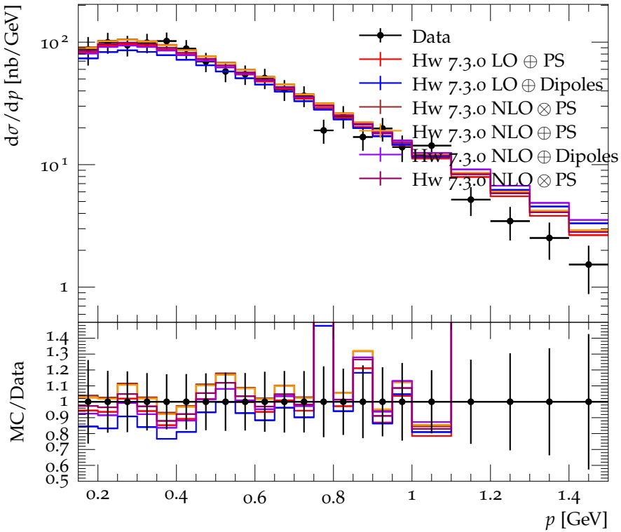
\pi^\pm momentum spectrum for E_{\text{CMS}} = 4.46 \rightarrow 4.98 GeV
