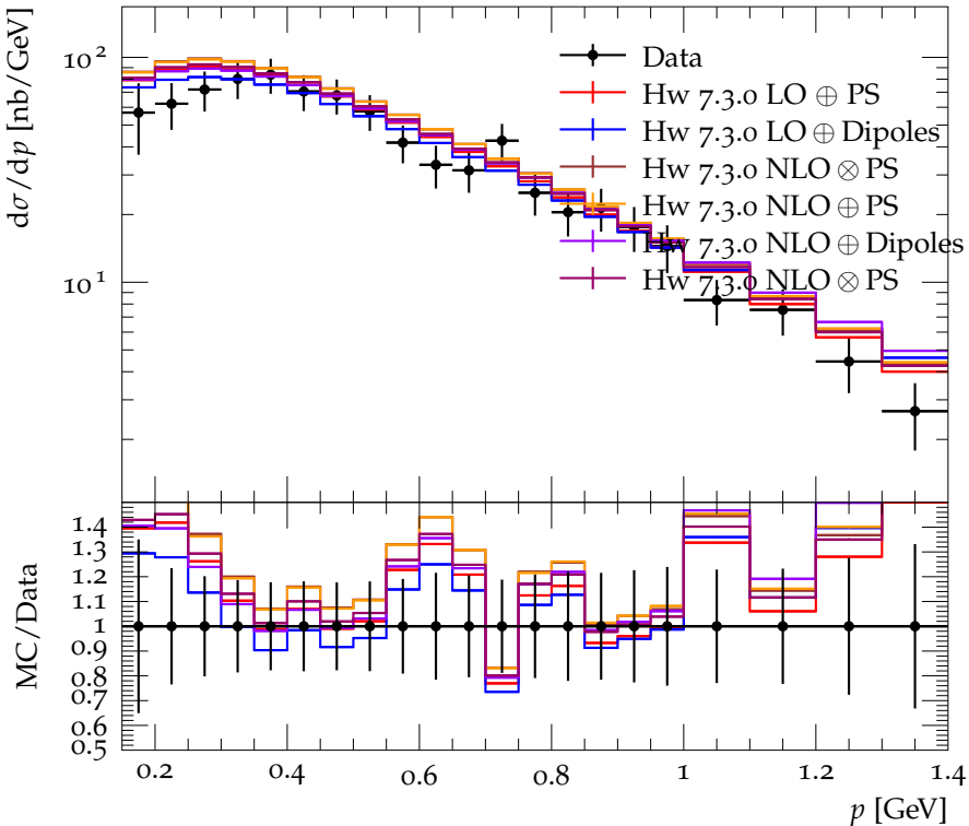
\pi^\pm momentum spectrum for E_{\text{CMS}} = 5.0 GeV
