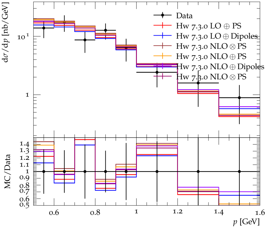
K^\pm momentum spectrum for E_{\text{CMS}} = 3.98 \rightarrow 4.10 GeV
