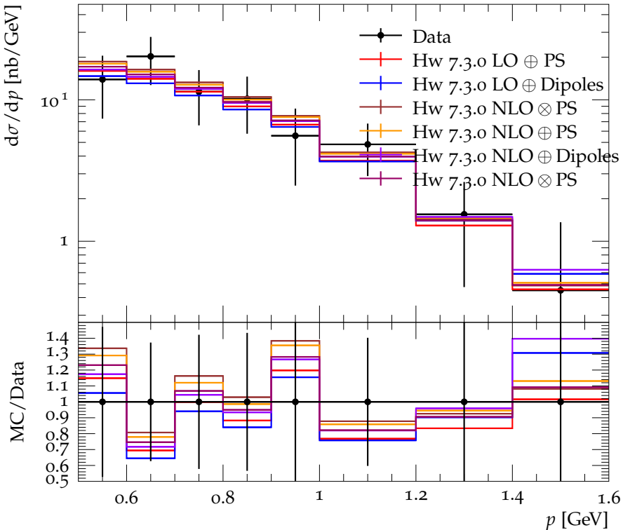
K^\pm momentum spectrum for E_{\text{CMS}} = 4.10 \rightarrow 4.24 GeV
