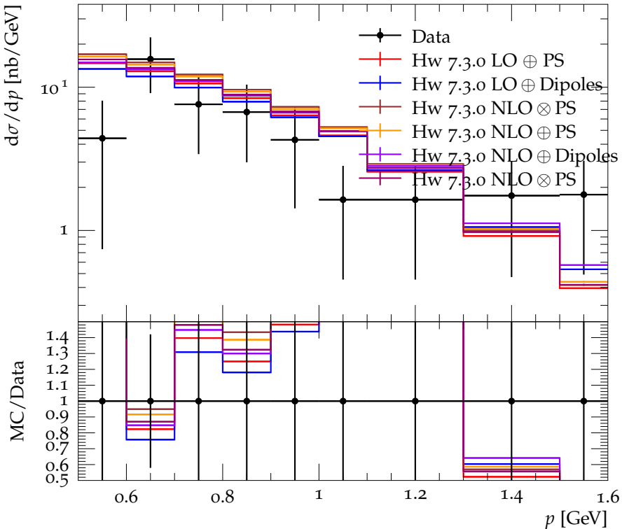
K^\pm momentum spectrum for E_{\text{CMS}} = 4.24 \rightarrow 4.36 GeV
