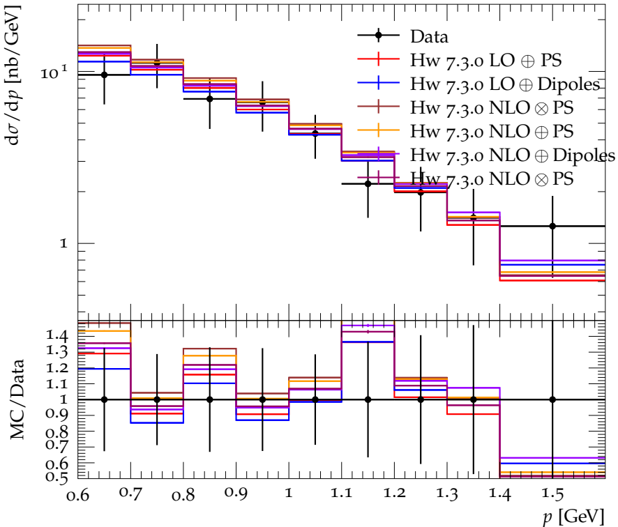
K^\pm momentum spectrum for E_{\text{CMS}} = 4.36 \rightarrow 4.46 GeV
