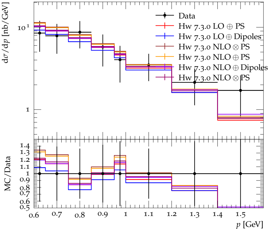
K^\pm momentum spectrum for E_{\text{CMS}} = 4.46 \rightarrow 4.98 GeV
