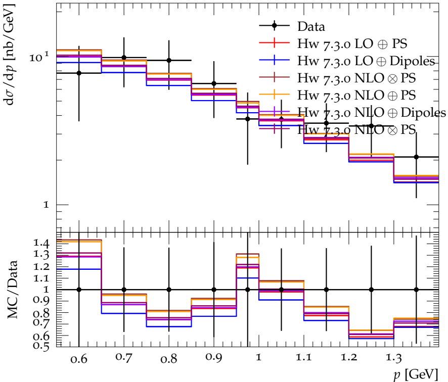
K^\pm momentum spectrum for E_{\text{CMS}} = 5.0 GeV
