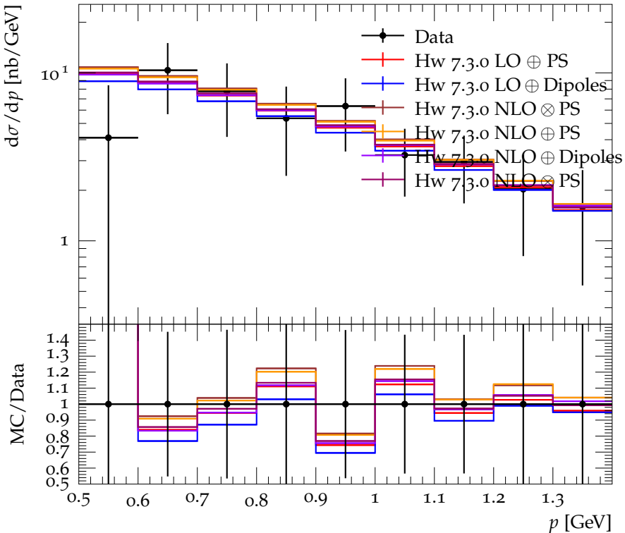
K^\pm momentum spectrum for E_{\text{CMS}} = 5.2 GeV
