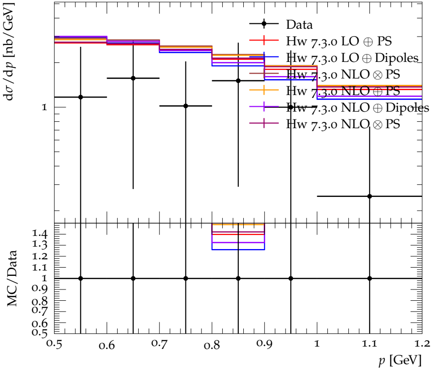
p, \bar{p} momentum spectrum for E_{\text{CMS}} = 5.0 GeV
