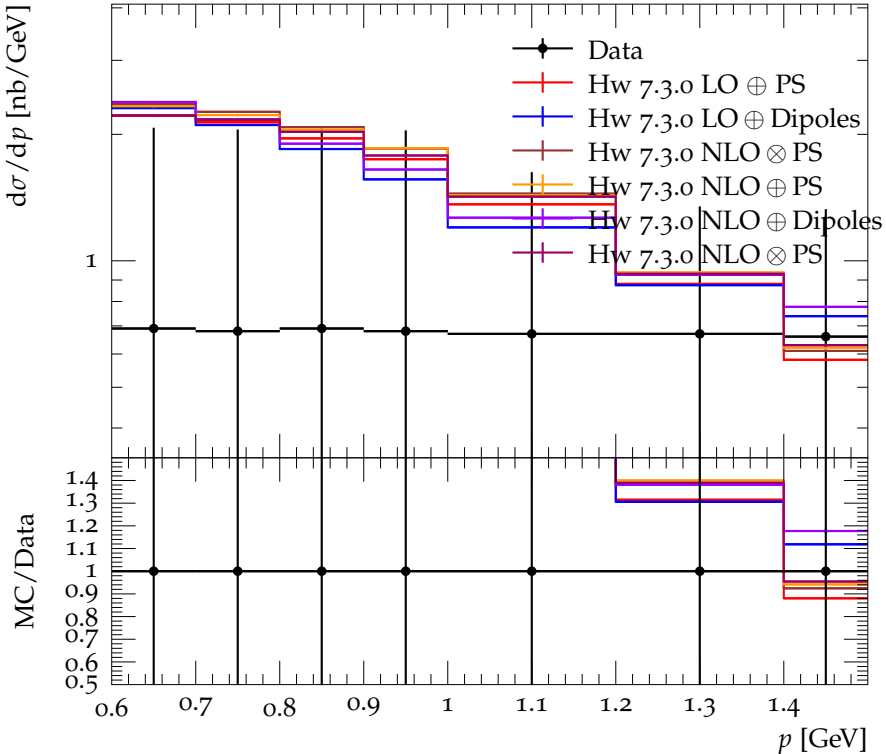
p, \bar{p} momentum spectrum for E_{\text{CMS}} = 5.2 GeV
