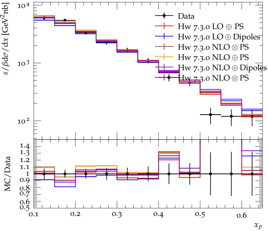
\pi^\pm scaled momentum spectrum for E_{\text{CMS}} = 5.0 GeV
