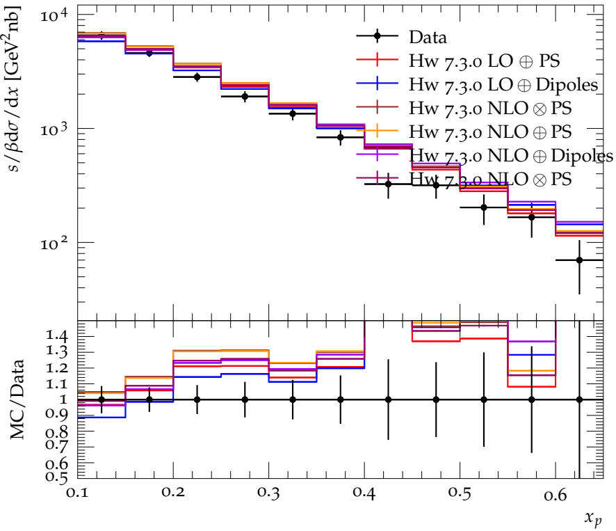
\pi^\pm scaled momentum spectrum for E_{\text{CMS}} = 5.2 GeV
