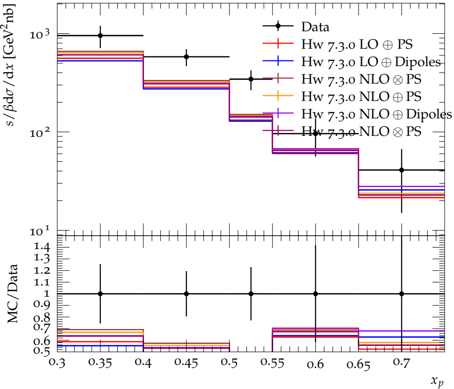
K^\pm scaled momentum spectrum for E_{\text{CMS}} = 3.98 \rightarrow 4.10 GeV
