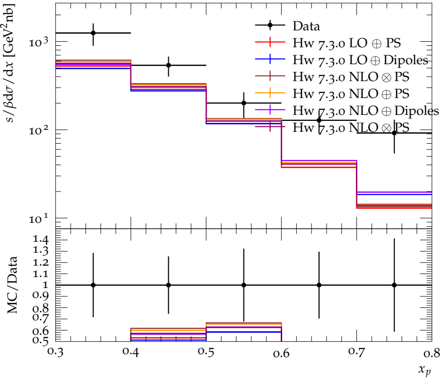
K^\pm scaled momentum spectrum for E_{\text{CMS}} = 4.10 \rightarrow 4.24 GeV
