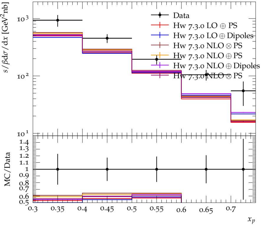
K^\pm scaled momentum spectrum for E_{\text{CMS}} = 4.36 \rightarrow 4.46 GeV
