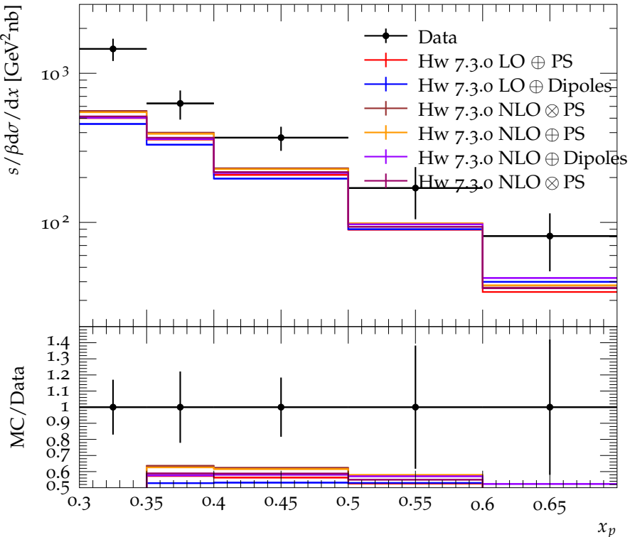
K^\pm scaled momentum spectrum for E_{\text{CMS}} = 4.46 \rightarrow 4.98 GeV
