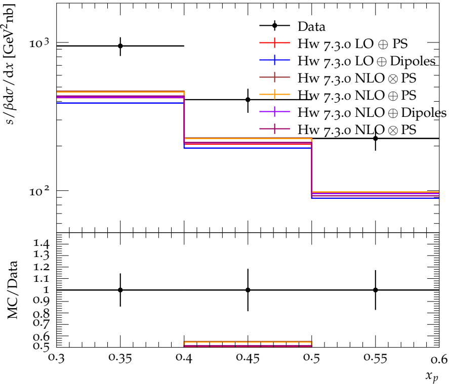
K^\pm scaled momentum spectrum for E_{\text{CMS}} = 5.0 GeV
