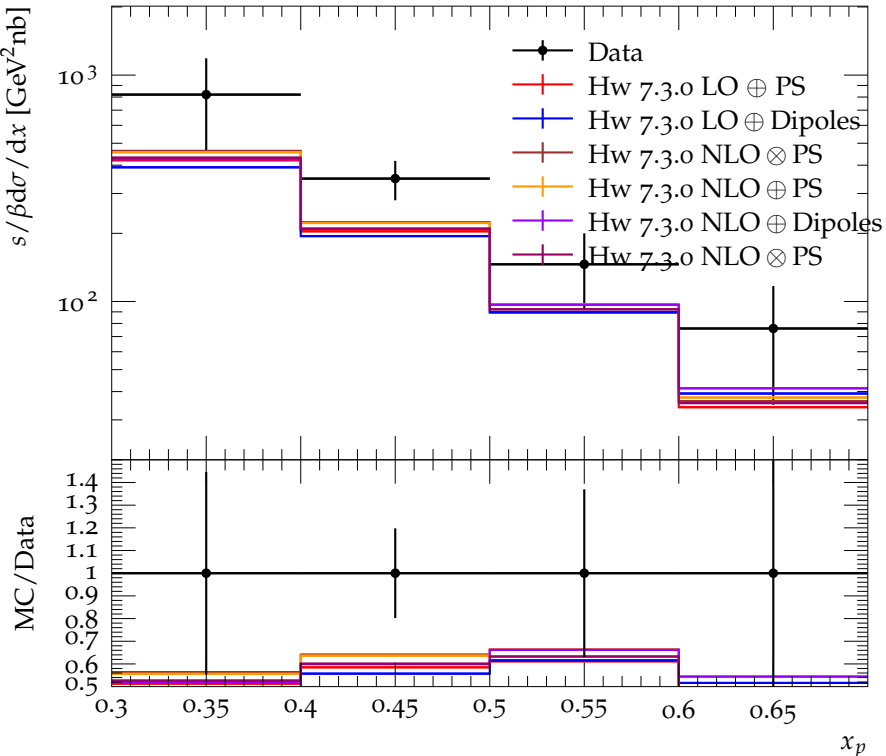
K^\pm scaled momentum spectrum for E_{\text{CMS}} = 5.2 GeV
