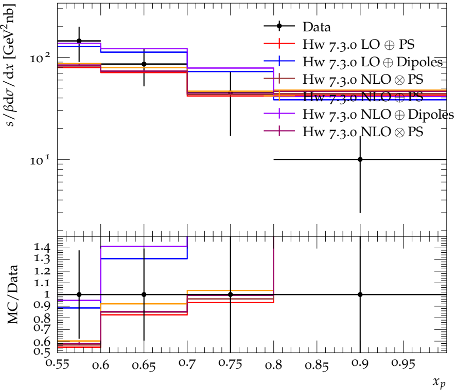
p, \bar{p} scaled momentum spectrum for E_{\text{CMS}} = 3.6 \rightarrow 3.67 GeV
