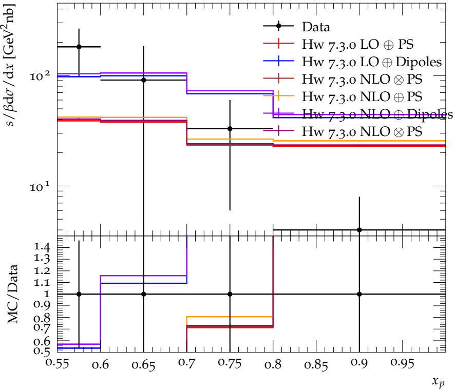
p, \bar{p} scaled momentum spectrum for E_{\text{CMS}} = 3.98 \rightarrow 4.10 GeV
