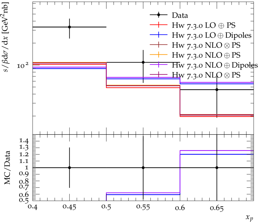
p, \bar{p} scaled momentum spectrum for E_{\text{CMS}} = 5.0 GeV
