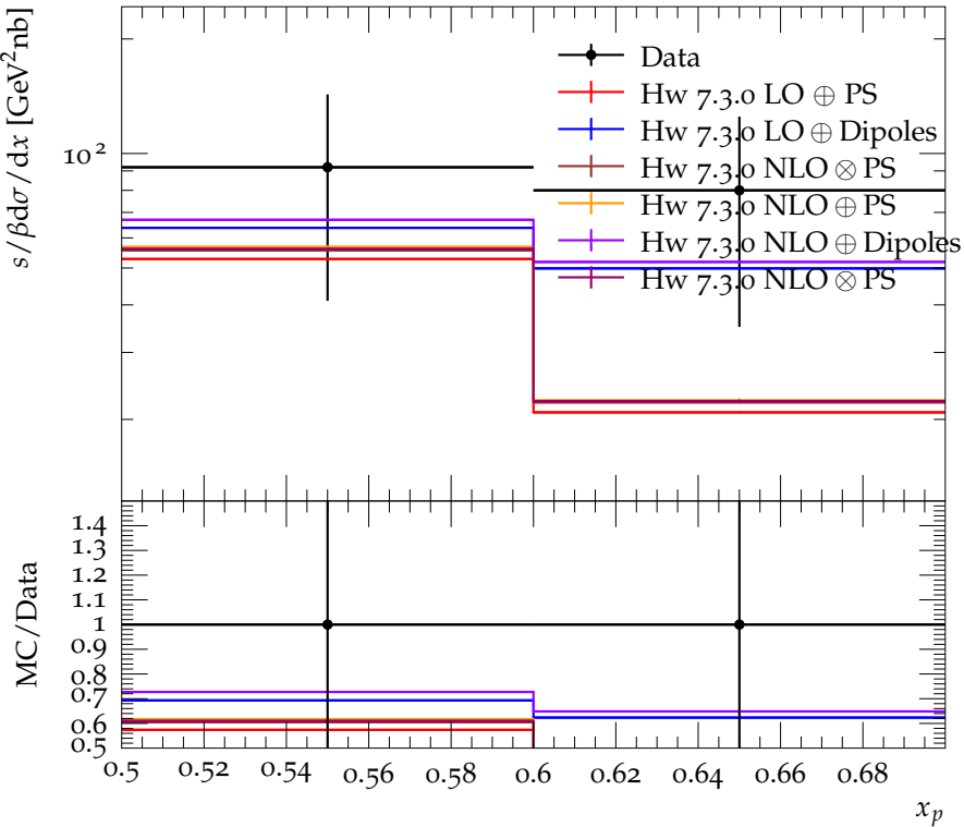
p, \bar{p} scaled momentum spectrum for E_{\text{CMS}} = 5.2 GeV
