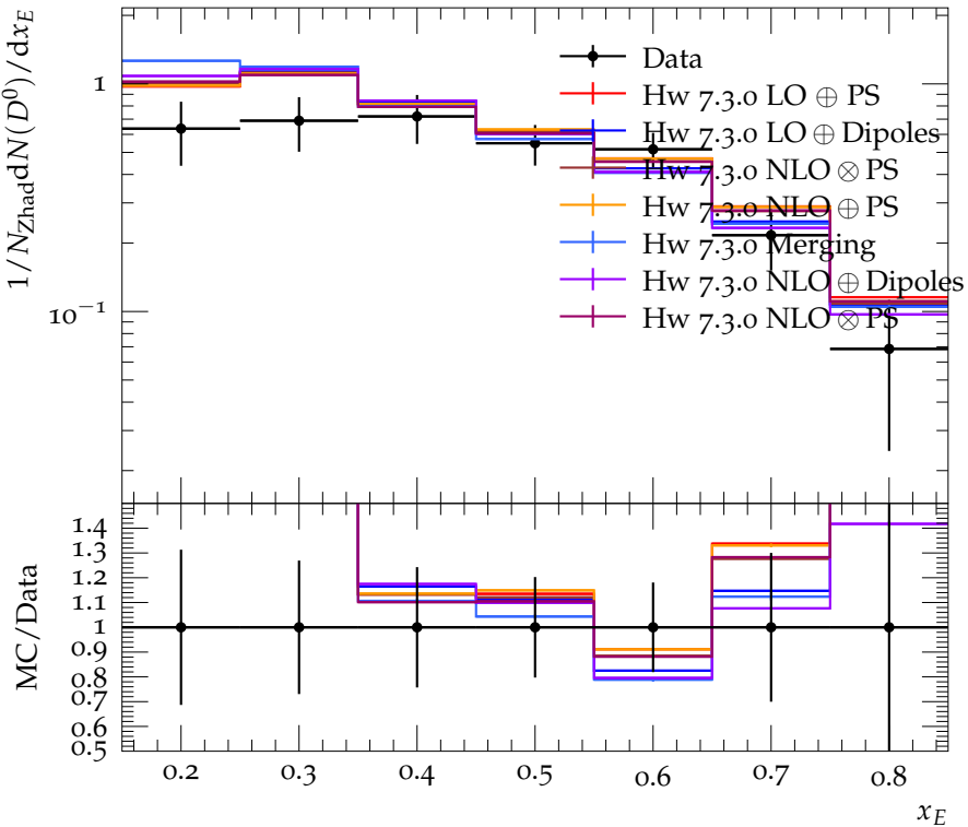
Scaled energy of D^0 at \sqrt{s} = 91.2 GeV
