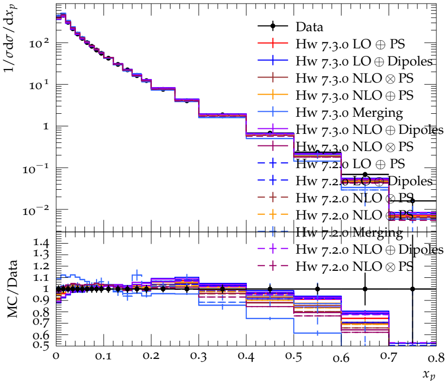
Charged Particle Scaled Momentum (bottom events)
