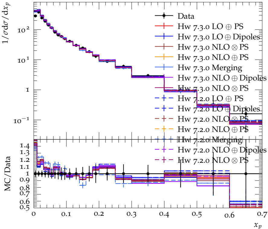
Charged Particle Scaled Momentum (charm events)
