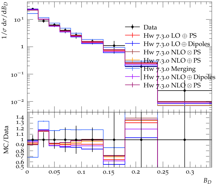
Difference of the jet broadenings ( E_{\text{CMS}} = 172 \text{ GeV} )
