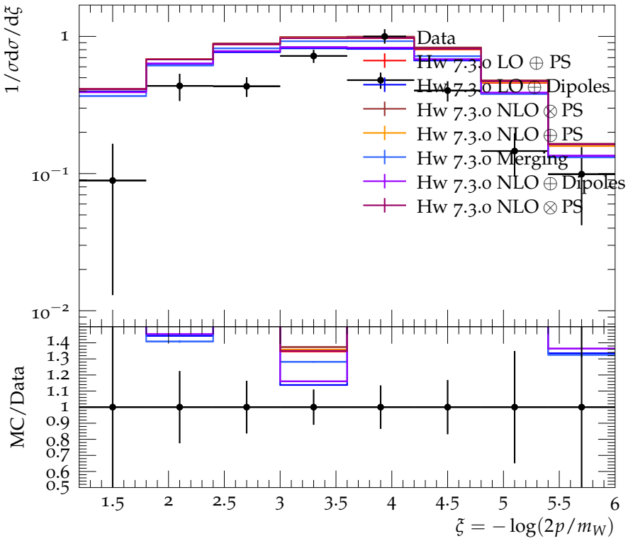
Log Scaled momentum fraction for K^0 at 183 GeV
