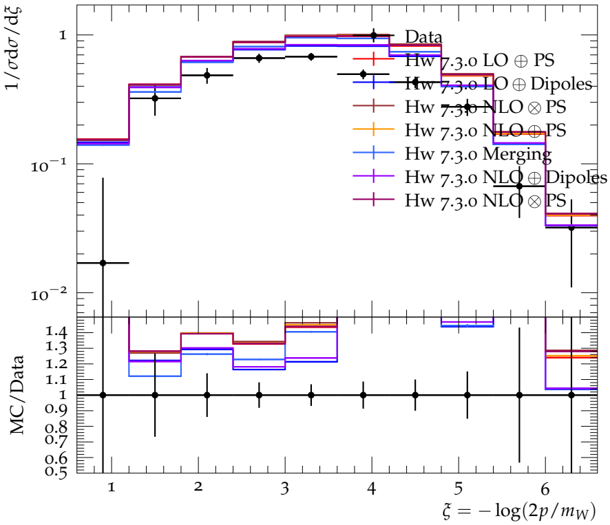
Log Scaled momentum fraction for K^0 at 189 GeV
