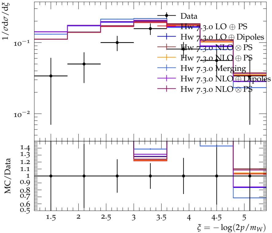
Log Scaled momentum fraction for \Lambda at 183 GeV
