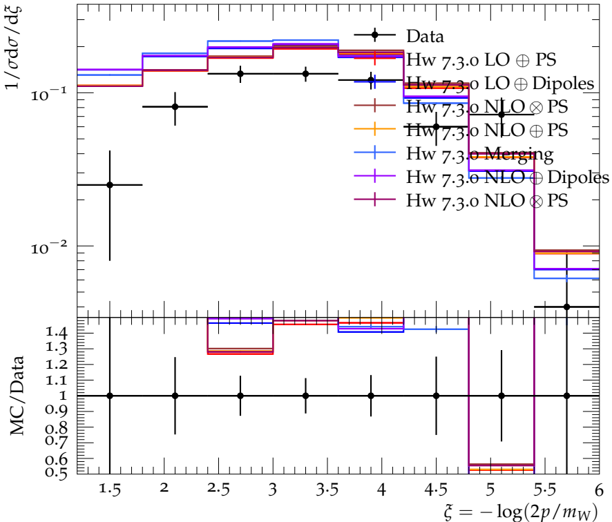
Log Scaled momentum fraction for \Lambda at 189 GeV
