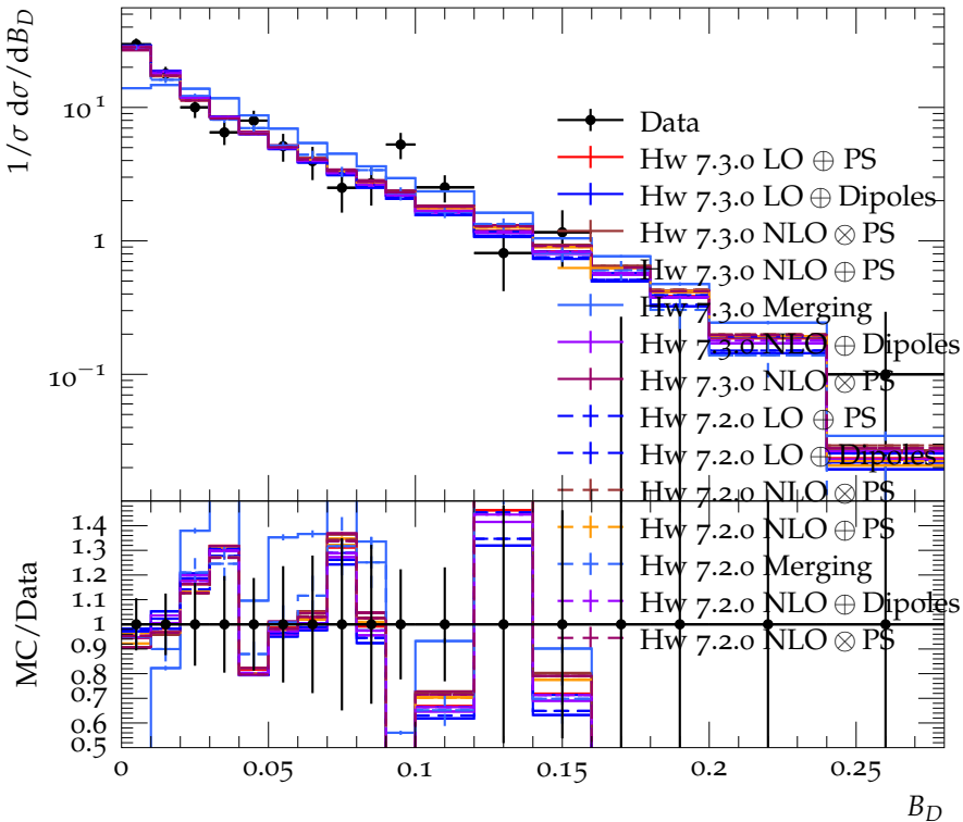
Difference of the jet broadenings ( E_{\text{CMS}} = 192 \text{ GeV} )
