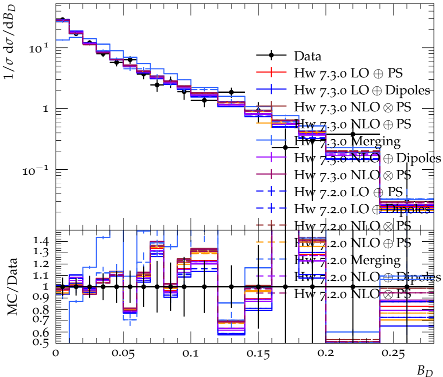
Difference of the jet broadenings ( E_{\text{CMS}} = 196 \text{ GeV} )
