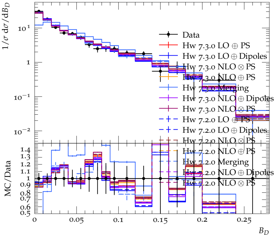
Difference of the jet broadenings ( E_{\text{CMS}} = 200 \text{ GeV} )
