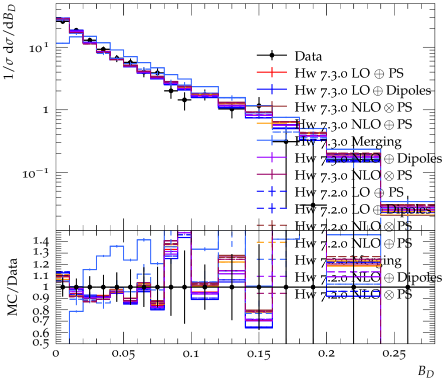
Difference of the jet broadenings ( E_{\text{CMS}} = 205 \text{ GeV} )
