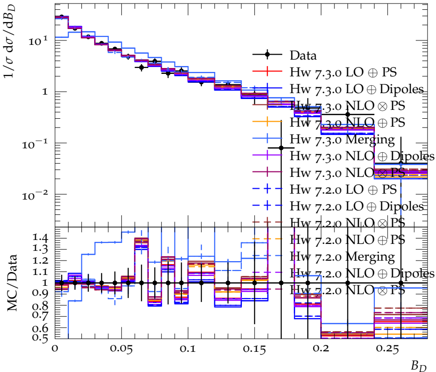
Difference of the jet broadenings ( E_{\text{CMS}} = 207 \text{ GeV} )
