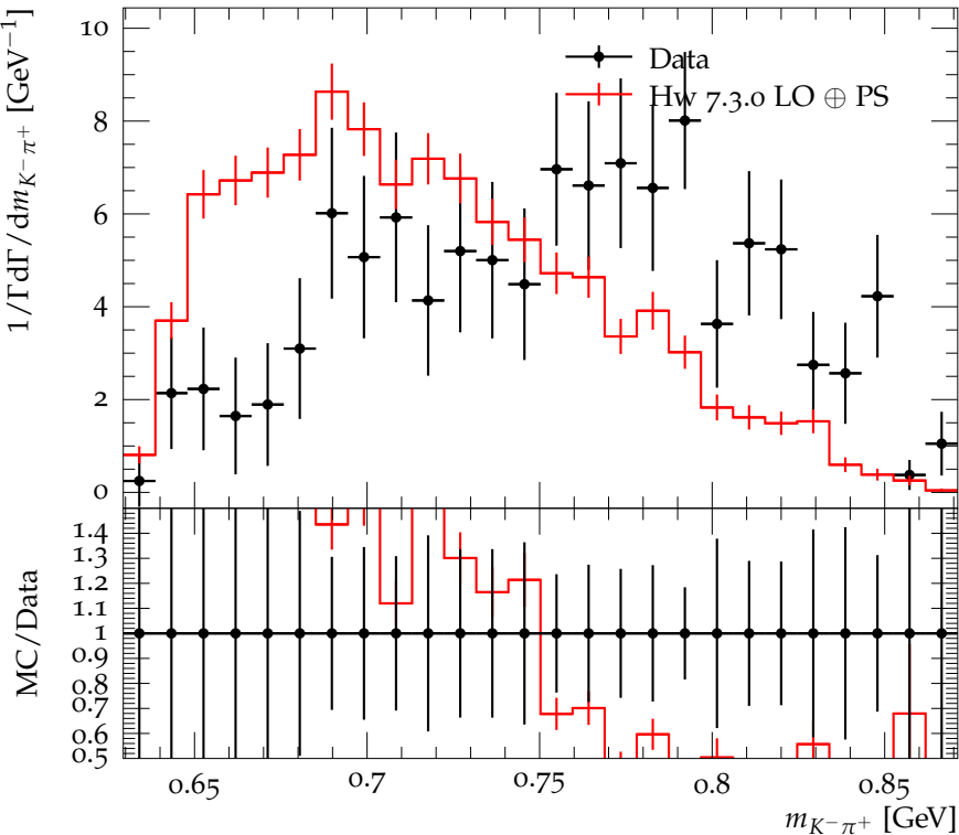
K^- \pi^+ mass distribution in D^0 \rightarrow K^- K^- K^+ \pi^+
