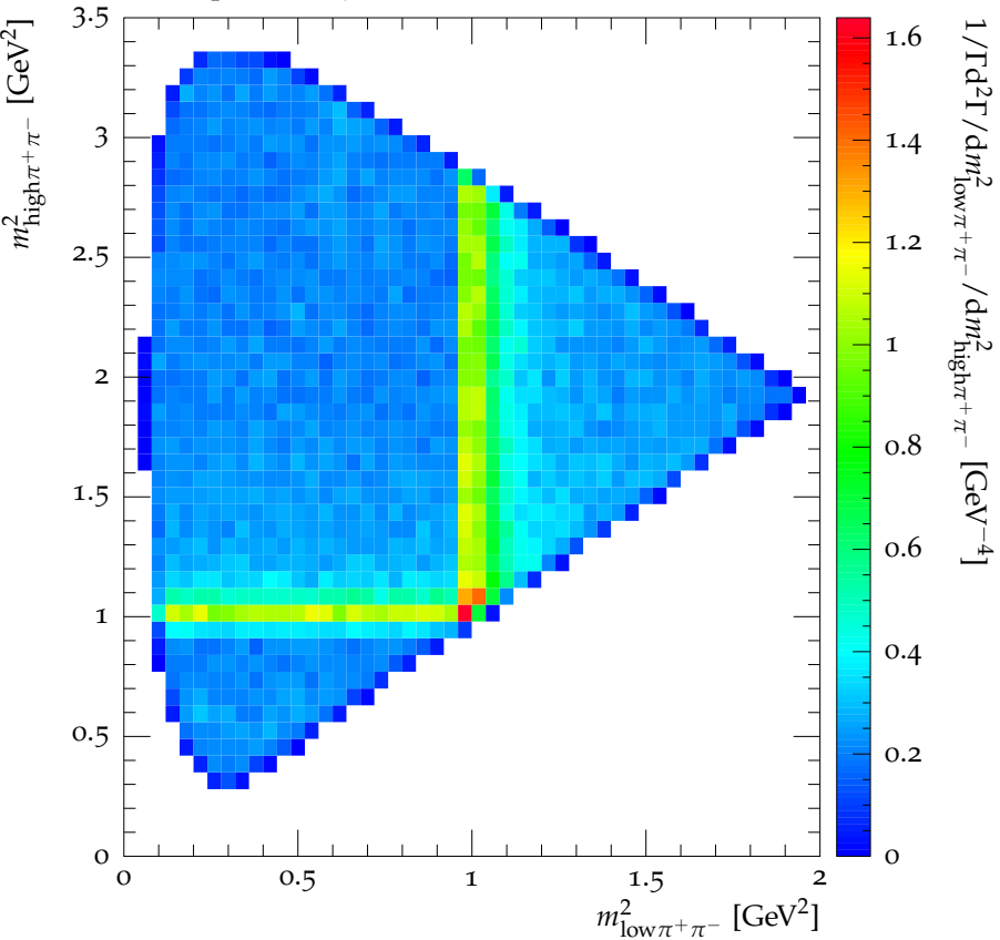
Dalitz plot for D_s^+ \rightarrow \pi^+ \pi^+ \pi^-
