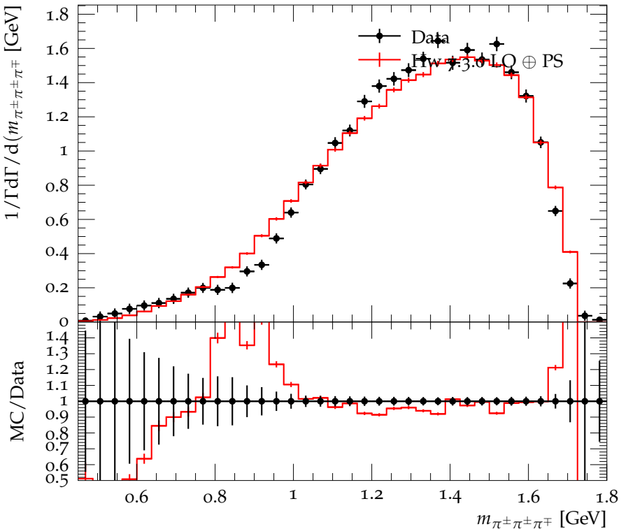
\pi^\pm\pi^\pm\pi^\mp mass distribution in D^0 \rightarrow 2\pi^+2\pi^-
