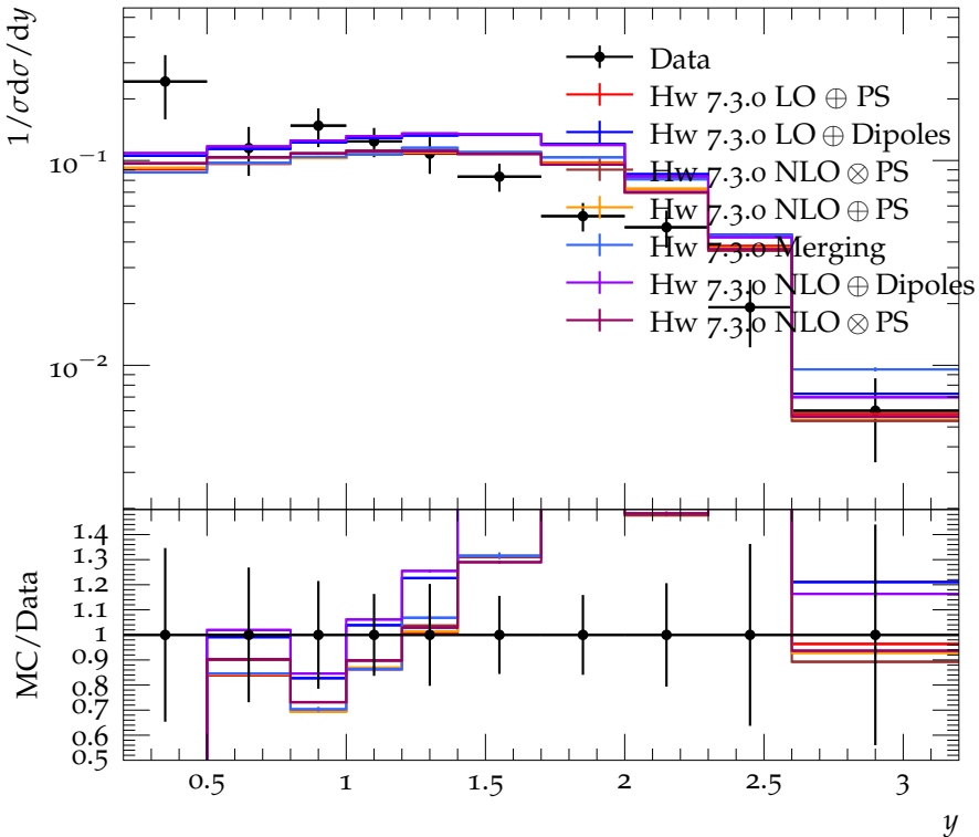
Rapidity w.r.t to thrust axis for \Lambda^0, \bar{\Lambda}^0 at 29 GeV
