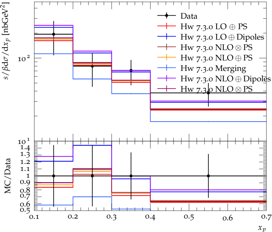
Scaled momentum for f_2(1270) at 29 GeV
