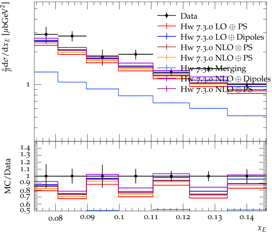
p, \bar{p} spectrum at 29 GeV
